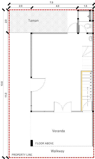
DENAH LANTAI 1 AL FRESCO VERANDA OPTION
