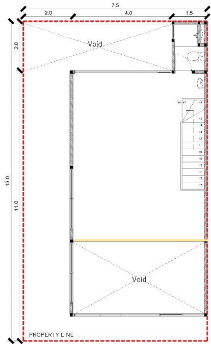
DENAH LANTAI 2
