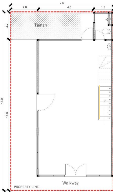
DENAH LANTAI 1 1 ST FLOOR FULL OPTION
