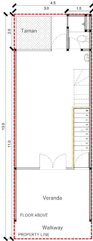
DENAH LANTAI 1 AL FRESCO VERANDA OPTION
