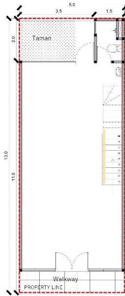
DENAH LANTAI 1 1 ST FLOOR FULL OPTION
