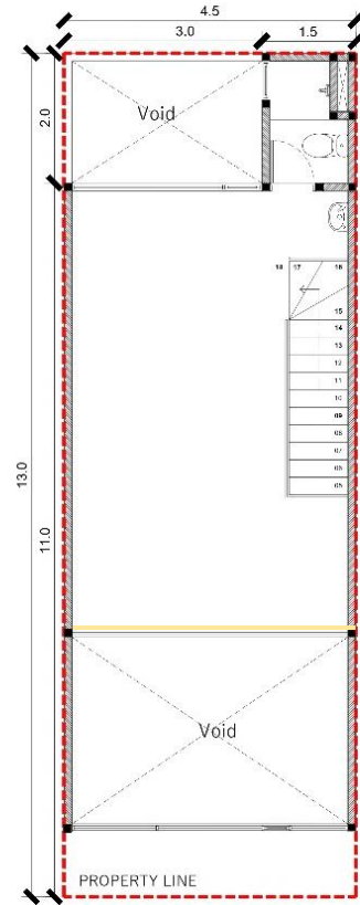
DENAH LANTAI 2
