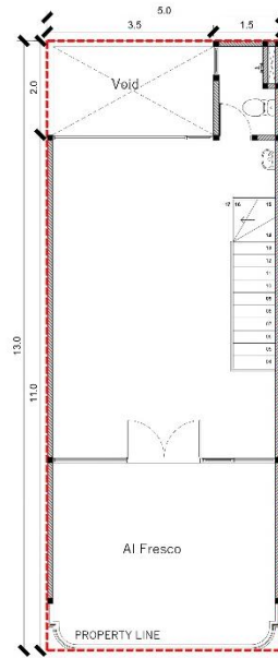
DENAH LANTAI 3
