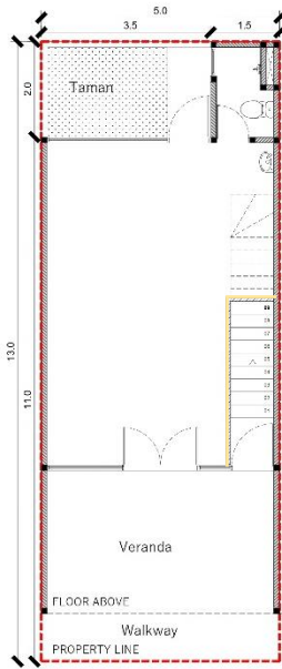
DENAH LANTAI 1 AL FRESCO VERANDA OPTION
