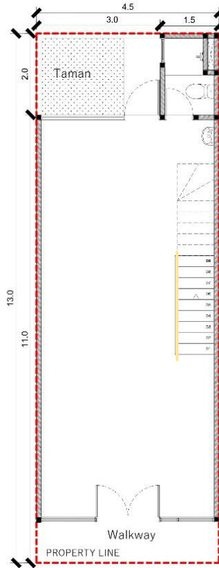
DENAH LANTAI 1 1 ST FLOOR FULL OPTION
