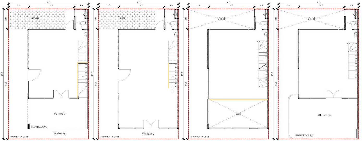
DENAH LANTAI 1 AL FRESCO VERANDA OPTION
